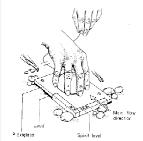
Figure 1. Placing hemisphere on the plane in a stream.
